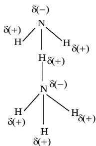
AMONIACO
